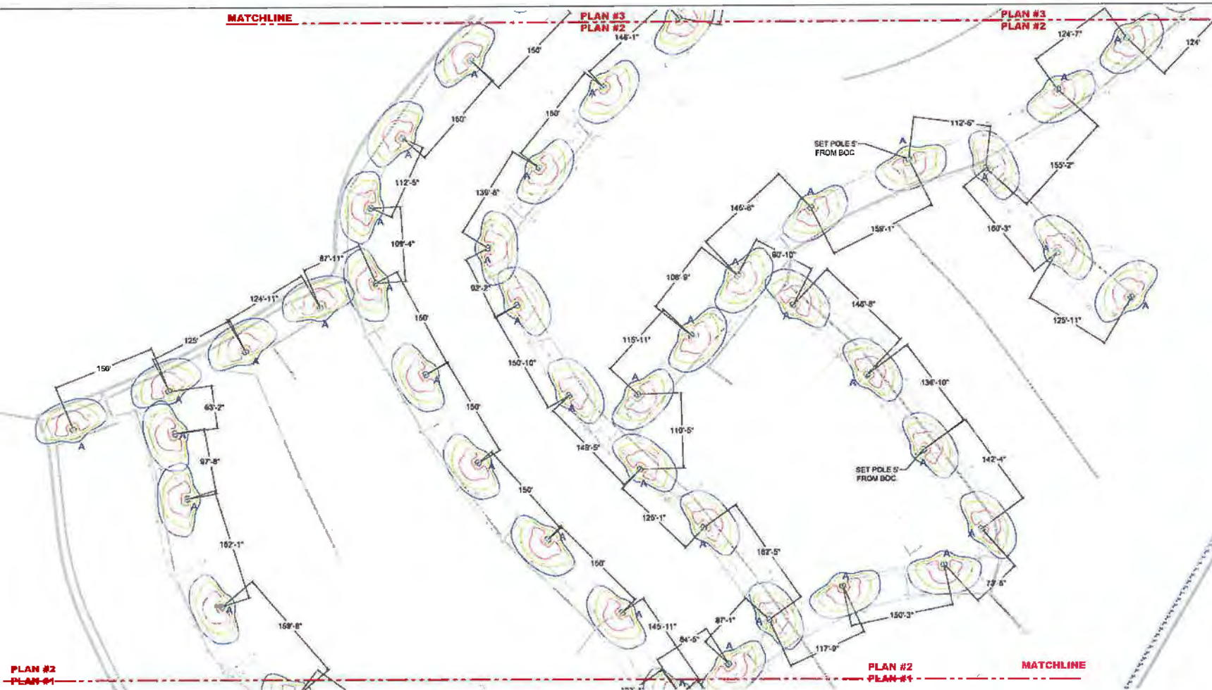
Site Photometry Plan #2 Scale: 1" = 60'
